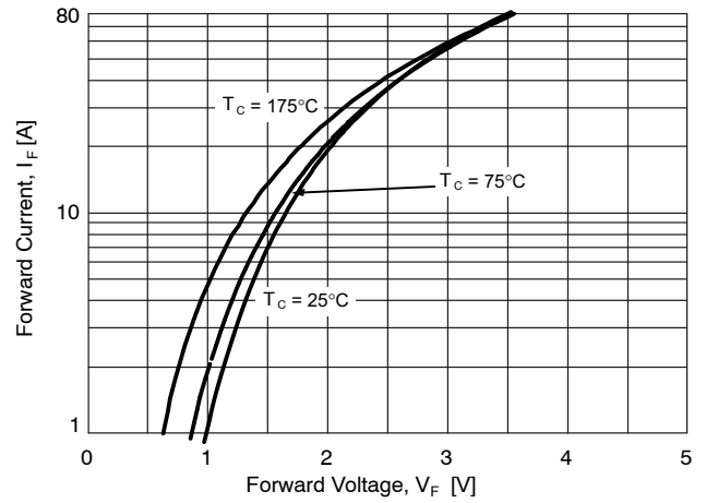
Figure 16. Forward Characteristics
