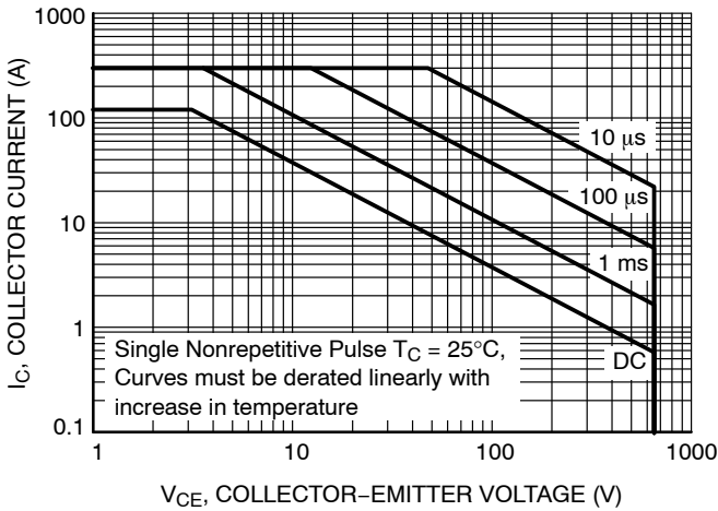
Figure 11. SOA Characteristics
